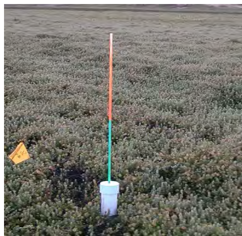
Fig. 1. Water level float installed on a commercial cranberry bog. Photo courtesy P. Jeranyama.
