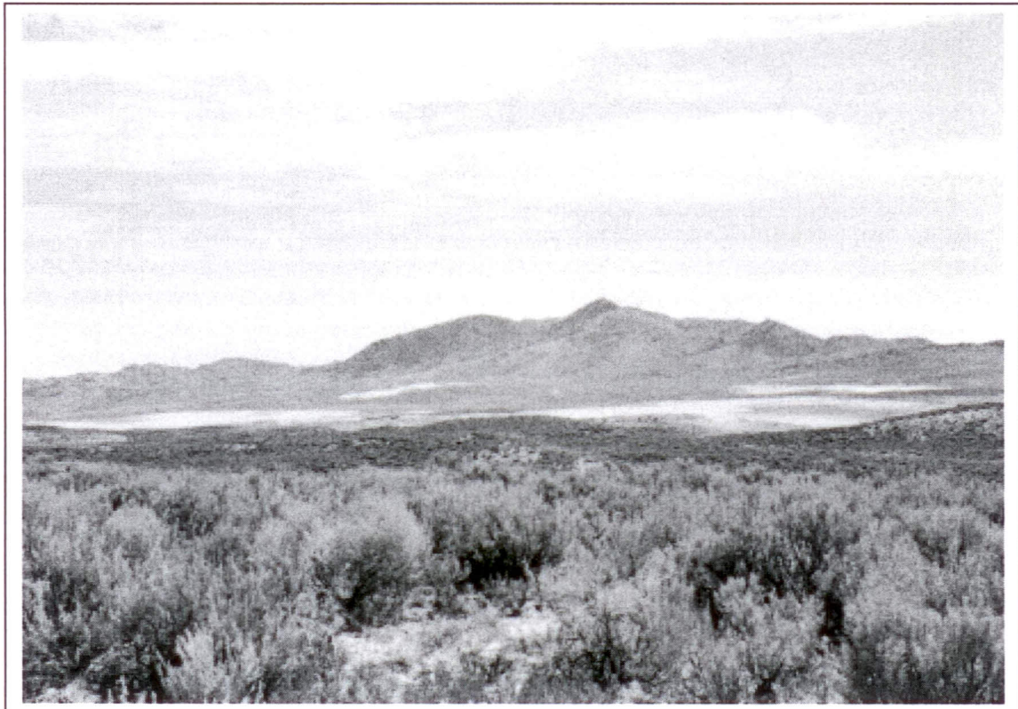
Figure 6. Habitat of Blowout penstemon on high sand dune on northwest flank of Bradley Peak (highest dune just to left of center of photo, below and to the left of the high point of Bradley Peak). Penstemon haydenii is absent from the lower elevation, rolling sand dunes in the middle foreground and from stabilized, sagebrush-dominated sand in the immediate foreground. WYNDD photo by Walter Fertig, 13 July 2000.
