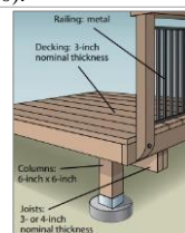
Figure 44. Deck constructed of heavy timber (FEMA, 2008a).
