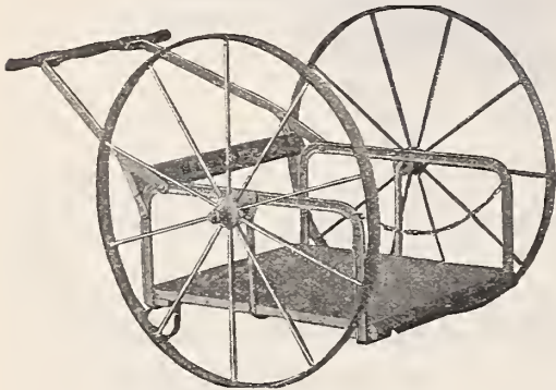
Size of platform 27x30 inches. Wheel 2-inch tire. Price, $12.00
