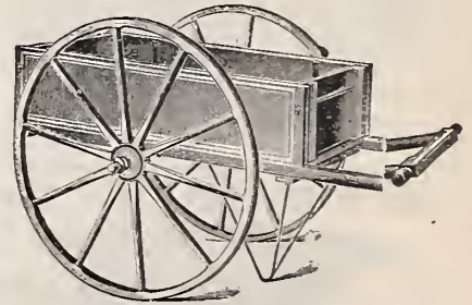
Tire, 1½ inches; wheel, 36 inches; axle, 1½ inches; hub, 6 inches.
