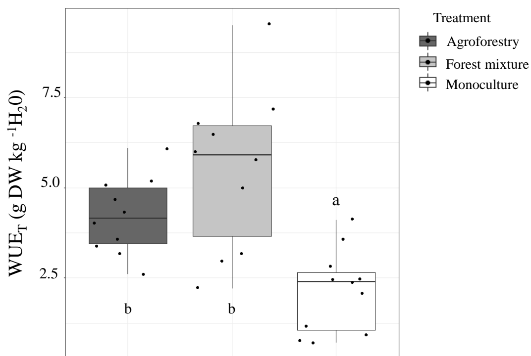
Figure 1. Transpiration efficiency ( WUE_T , g DW kg -1 H 2 O) for poplars in different treatments (n = 12) during the 2020 growing season (June to September). Different letters indicate significant differences between treatments.
