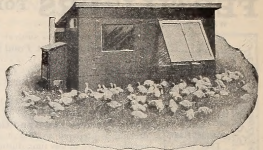
THE NEW PRAIRIE STATE COMBINATION COLONY BROODER.
