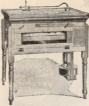
THE NEW PRAIRIE STATE JUNIOR No. 1 INCUBATOR.
