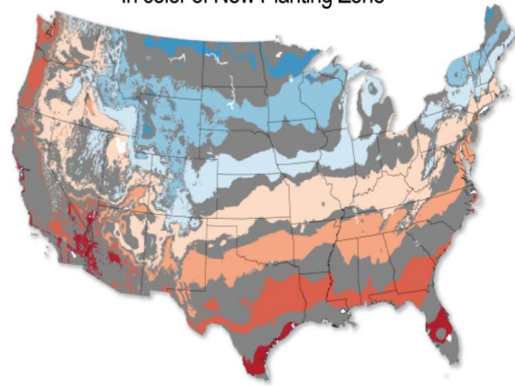
Average Annual Extreme Minimum Temperature by Climate-Related Planting Zone
