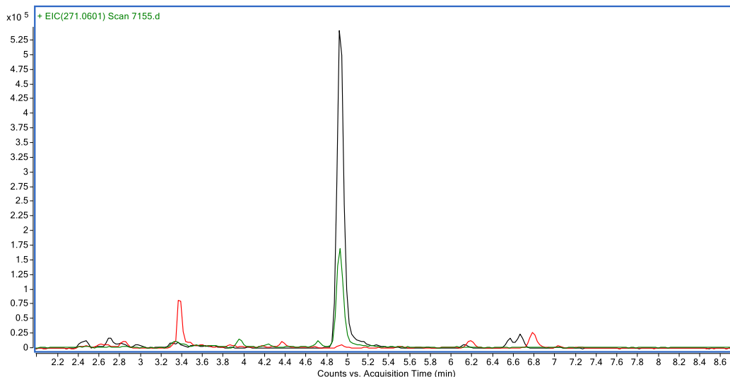
Sorbus dacica
