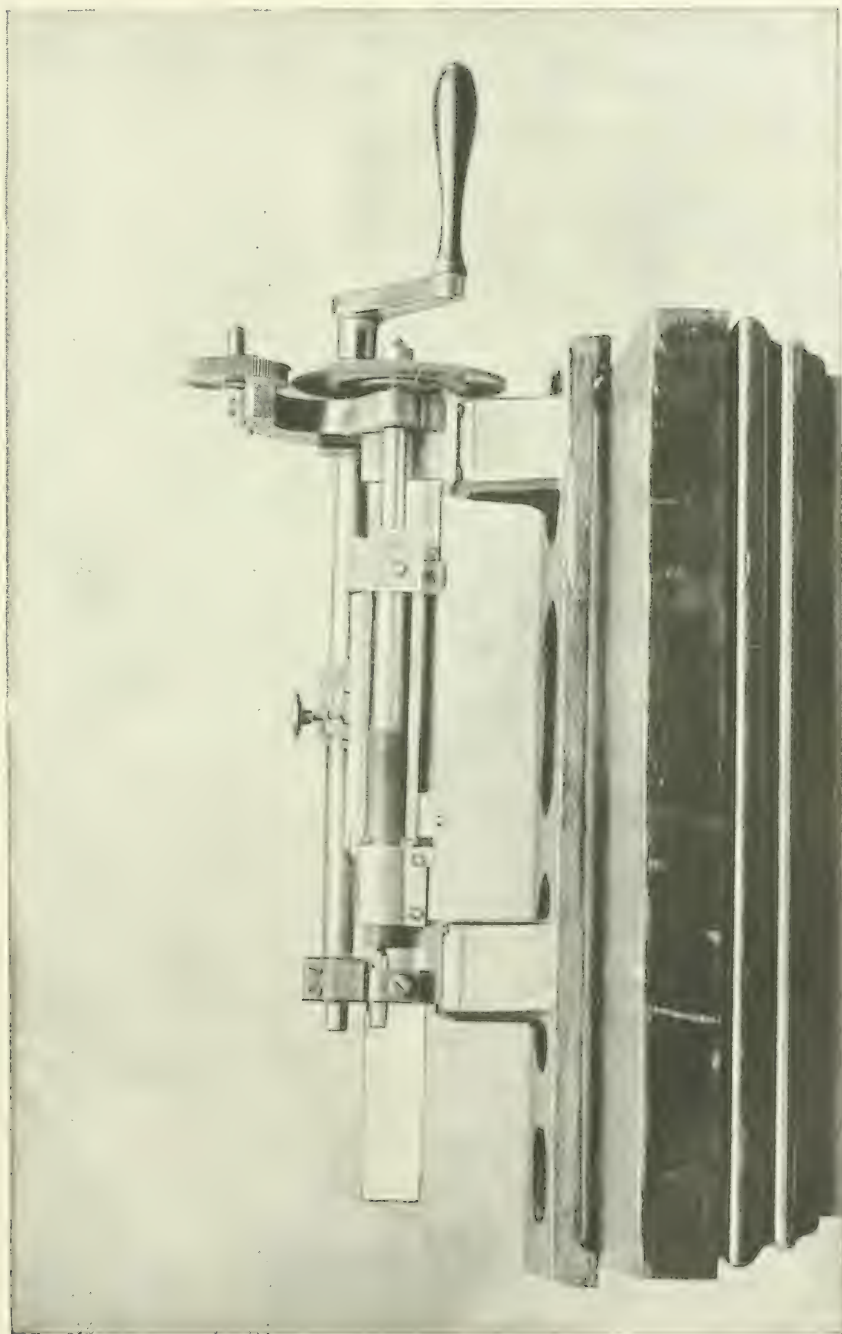
MACHINE BY WHICH THE ENIGMA SKEW AND THE TEETH IN THE PLATE OF THE RASDEN DENTAL ENGINE WERE CUT.
