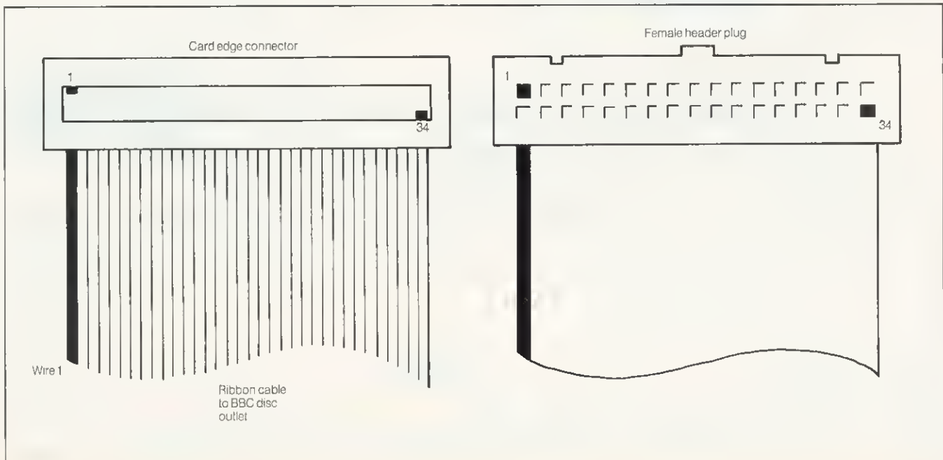
Below: Front view of connectors for disc cable
