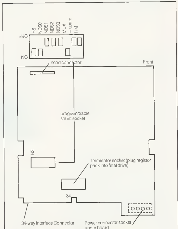
Top view of Tandem disc drive PCB
