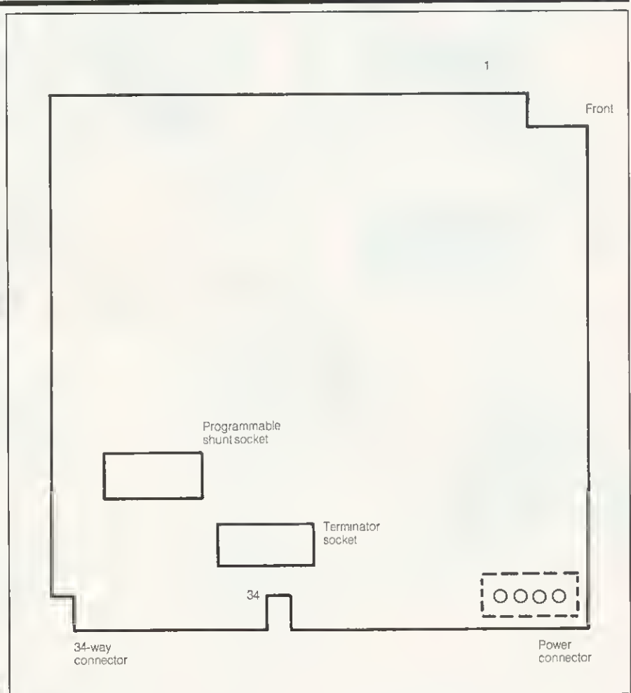
Above: Top view of Control Data drive PCB
